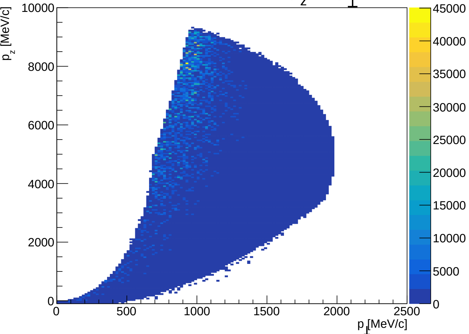
Scattered electron p_z vs p_\perp
