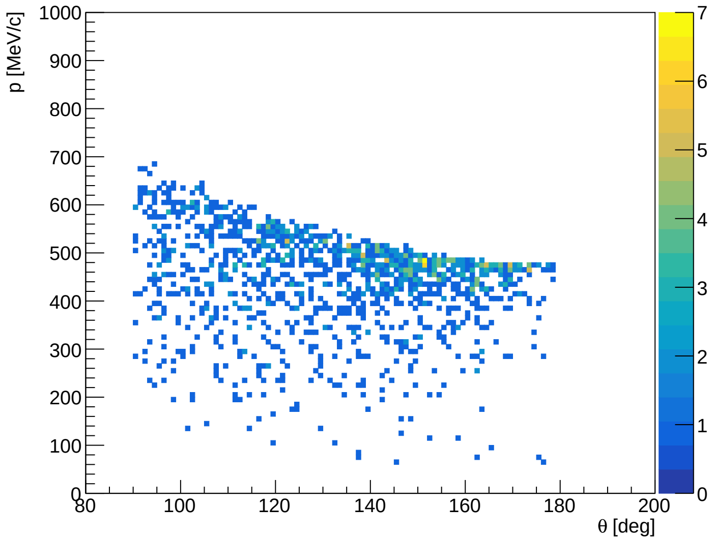
HMS accepted recoil particle p vs \theta
