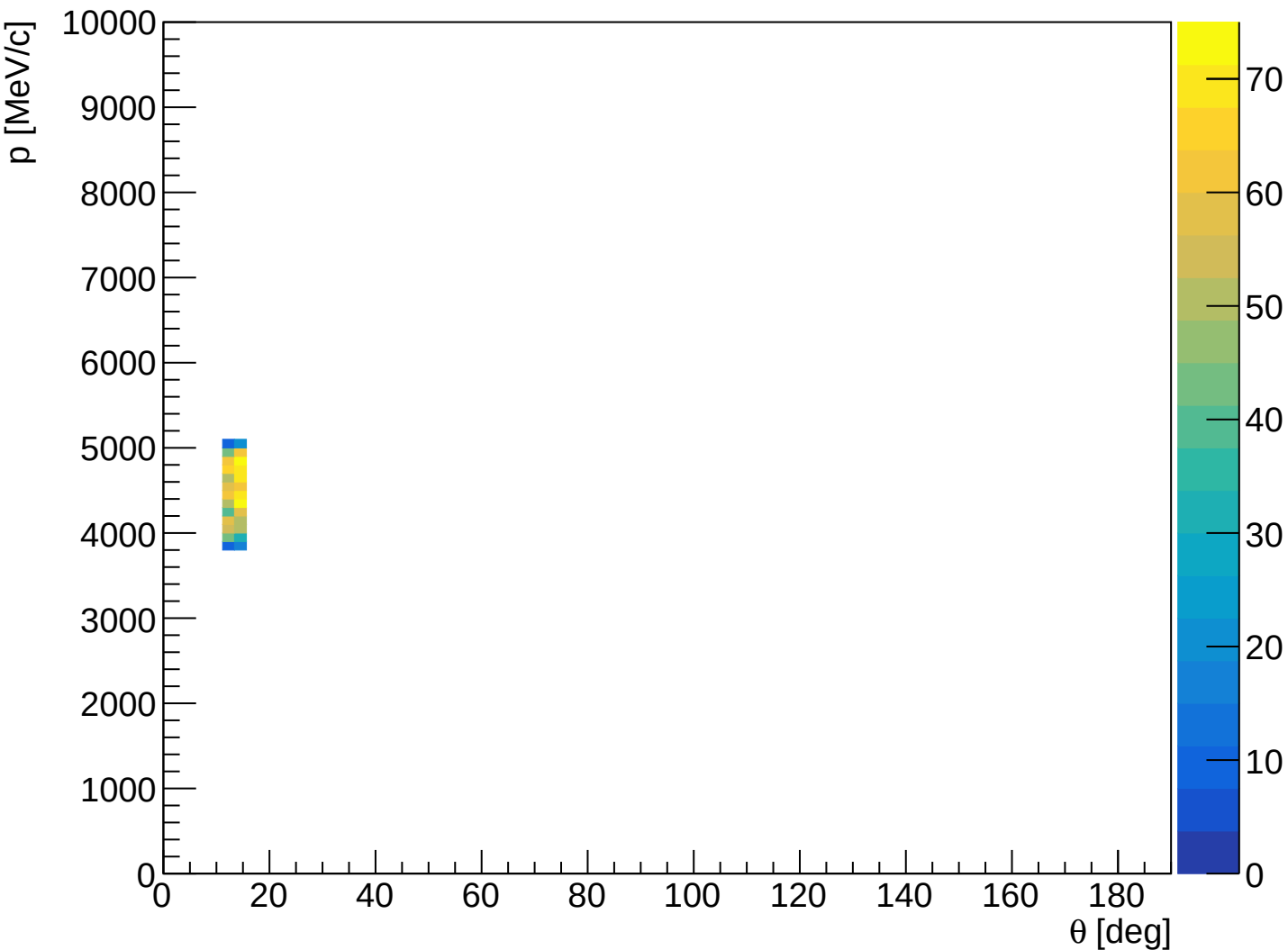
HMS accepted scattered electron p vs \theta
