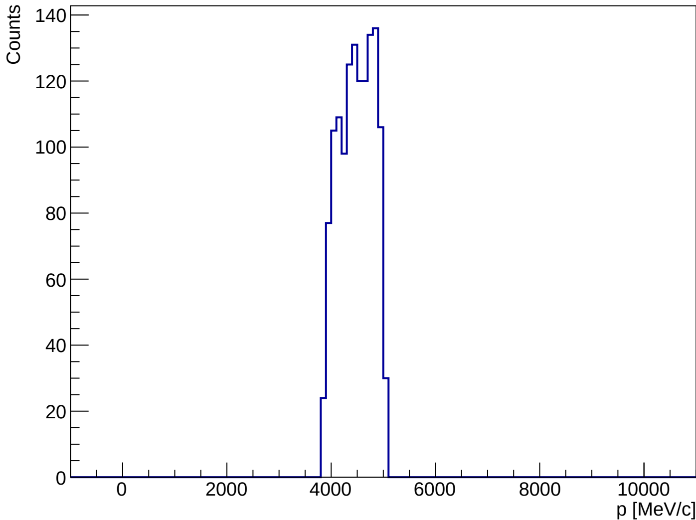
HMS accepted scattered electron momentum magnitude
