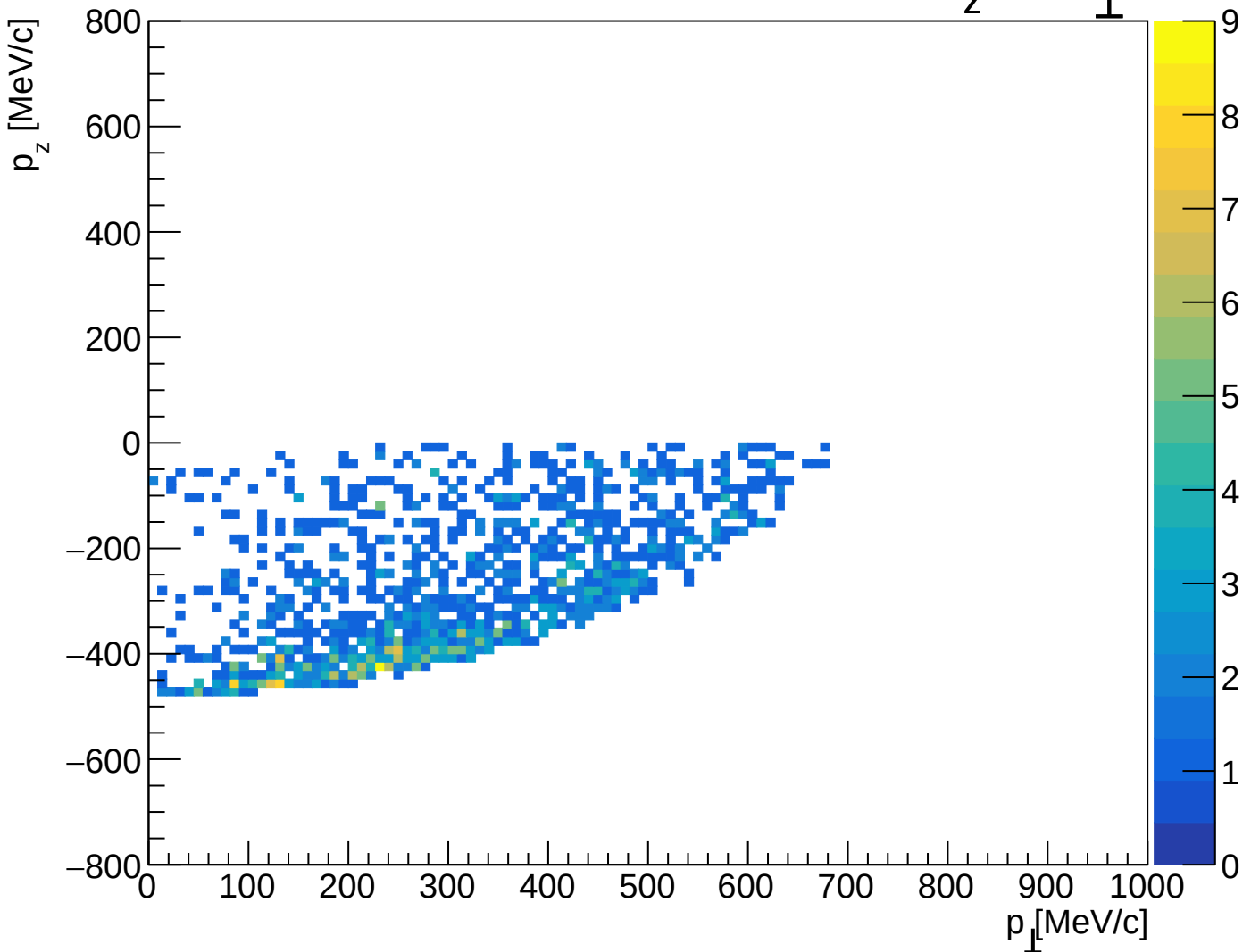
HMS accepted recoil particle p_z vs p_\perp
