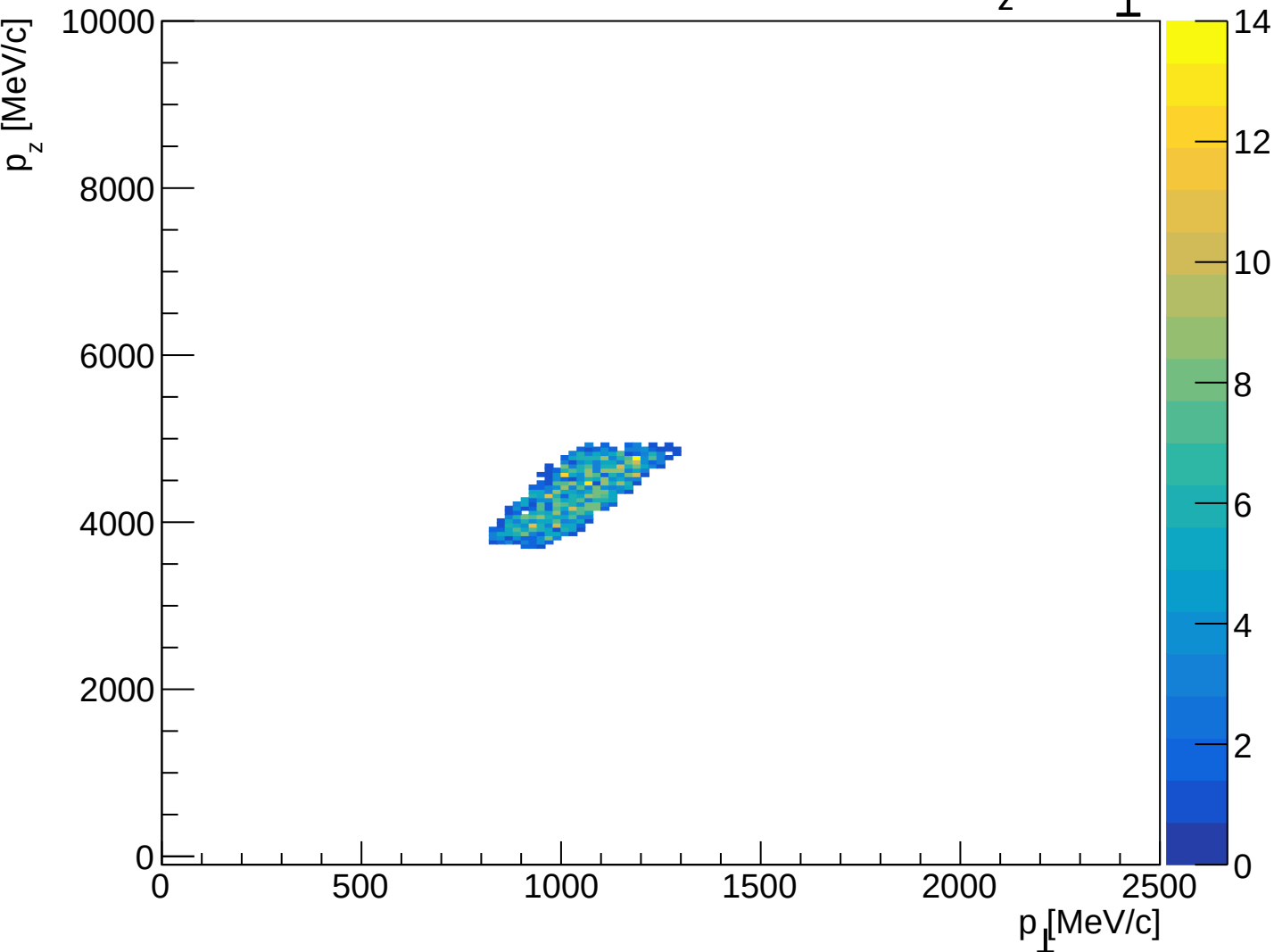
HMS accepted scattered electron p_z vs p_\perp
