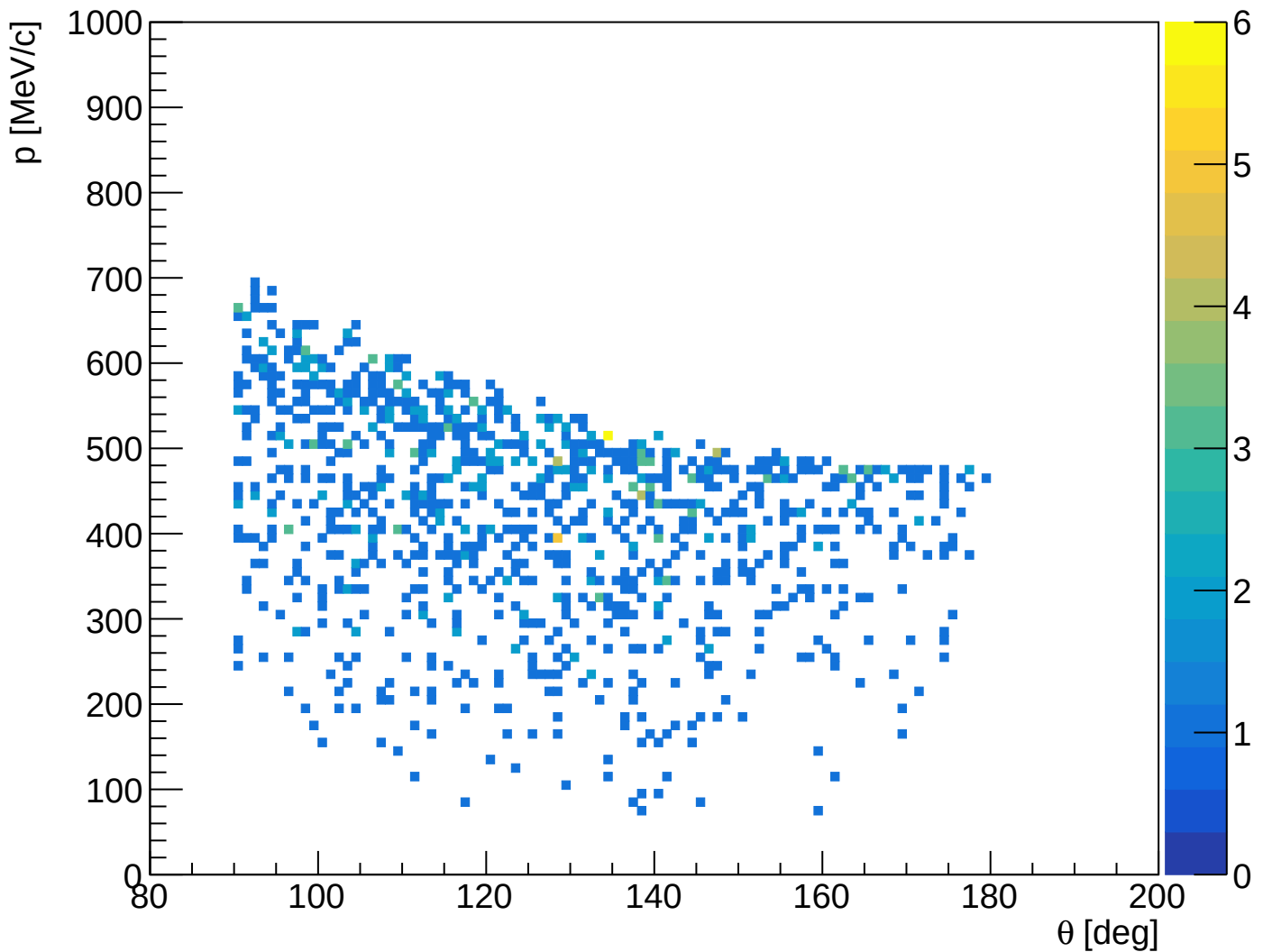
SHMS accepted recoil particle p vs \theta
