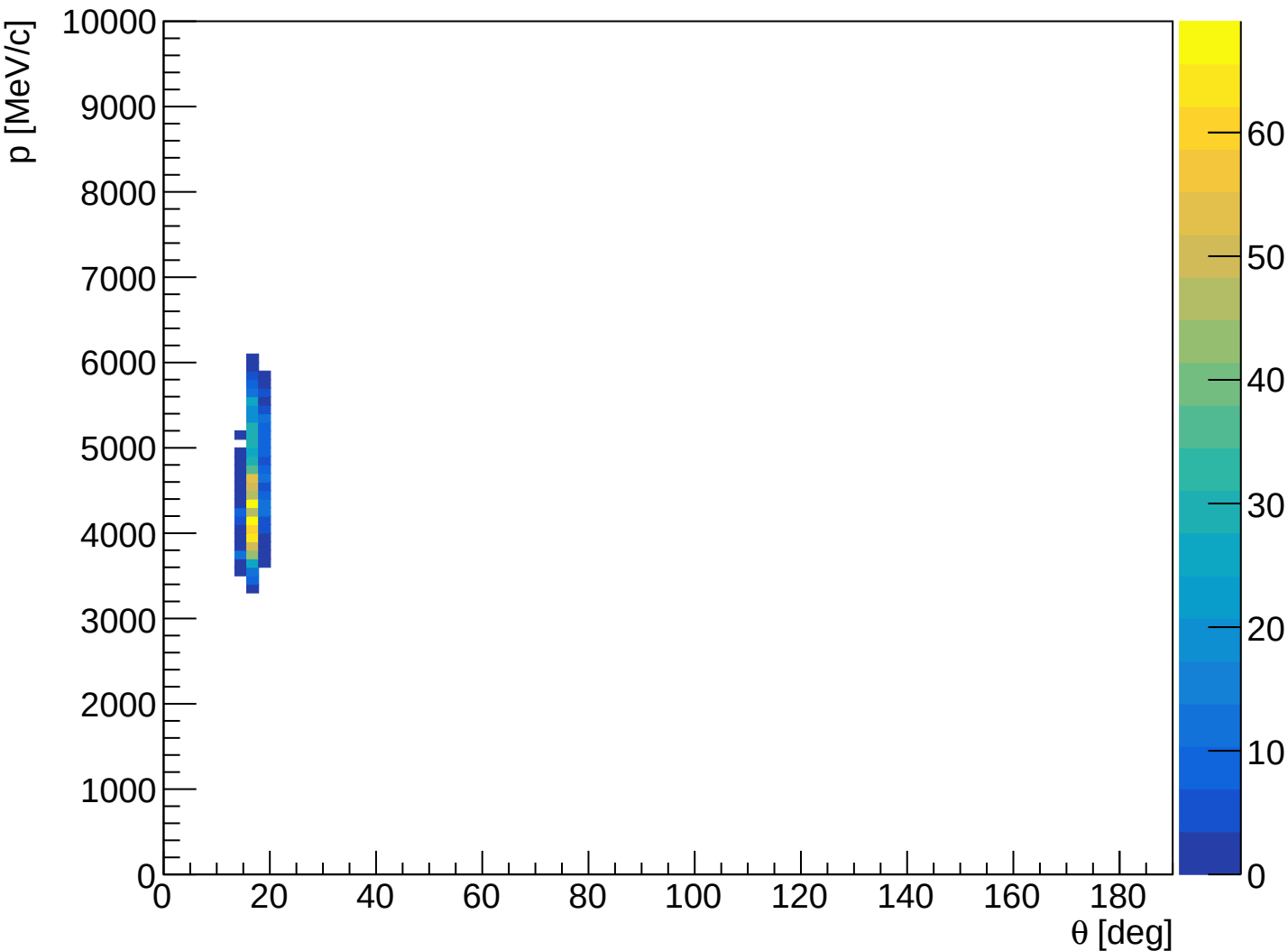
SHMS accepted scattered electron p vs \theta
