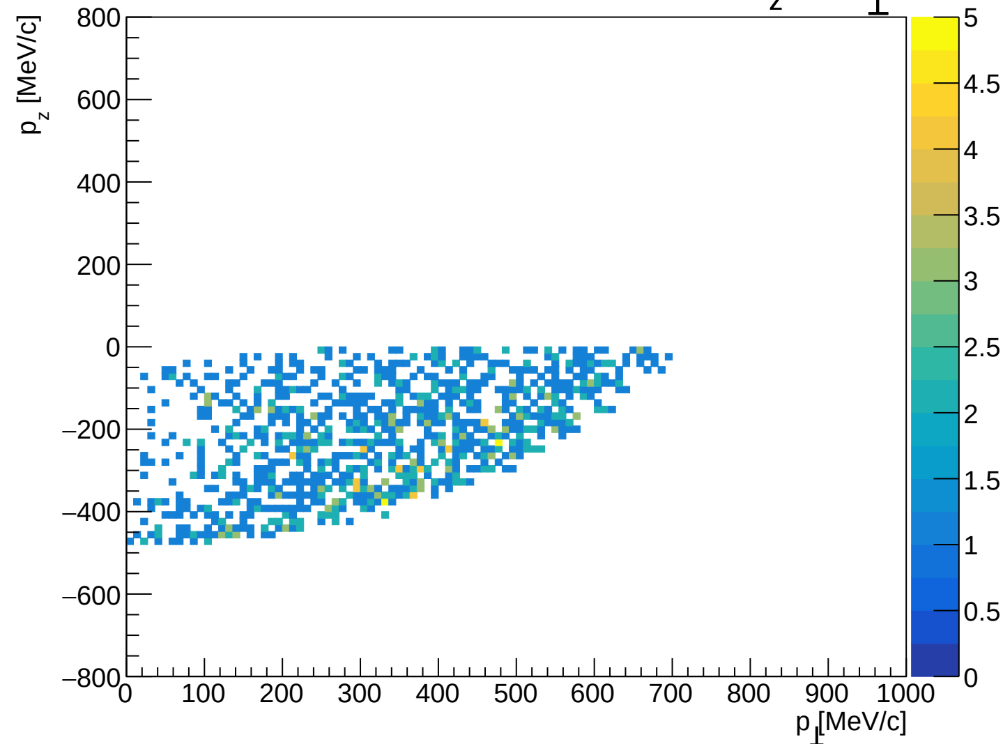
SHMS accepted recoil particle p_z vs p_\perp
