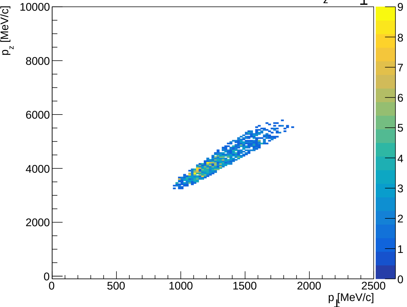
SHMS accepted scattered electron p_z vs p_\perp
