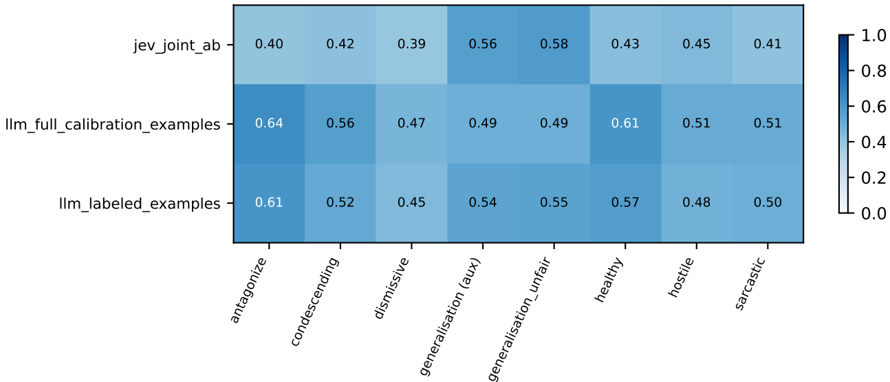
adaptation_discovery_v1 / ucc / discovery: Fixed-original-class macro F1
