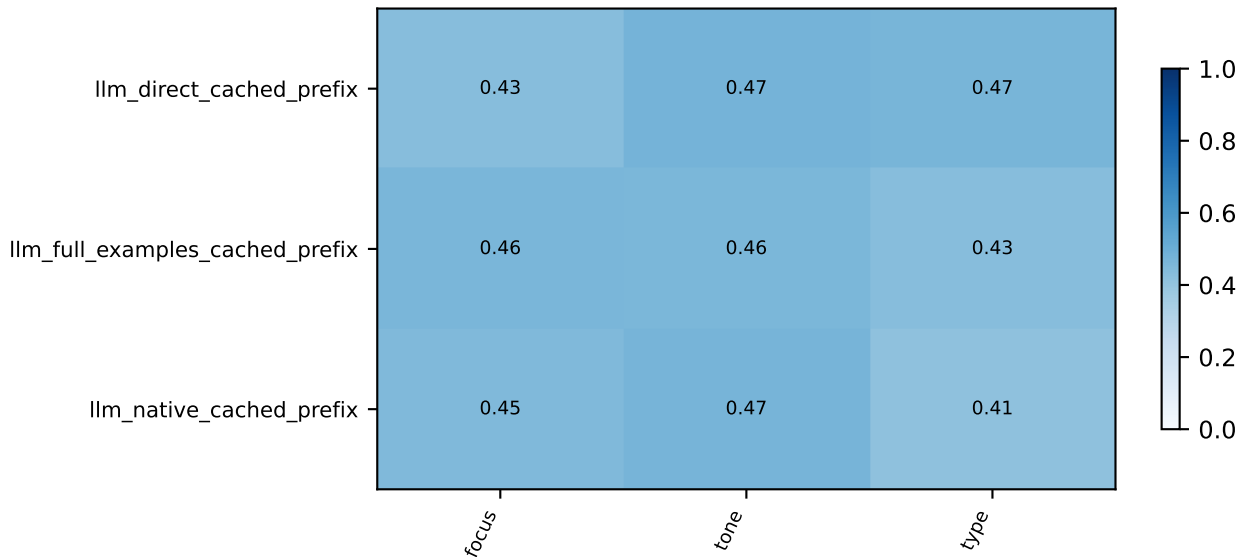
cache_prefix_diagnostic_v1 / mbd / diagnostic: Fixed-original-class macro F1
