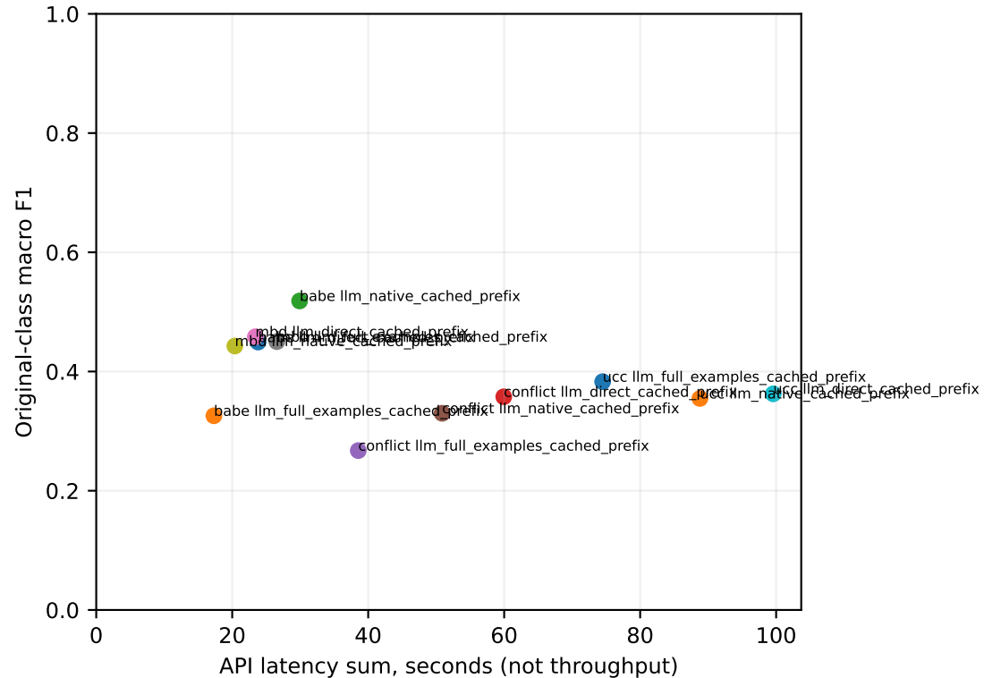
cache_prefix_diagnostic_v1 efficiency-quality tradeoffs
