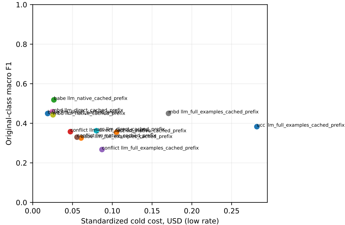
cache_prefix_diagnostic_v1 efficiency-quality tradeoffs
