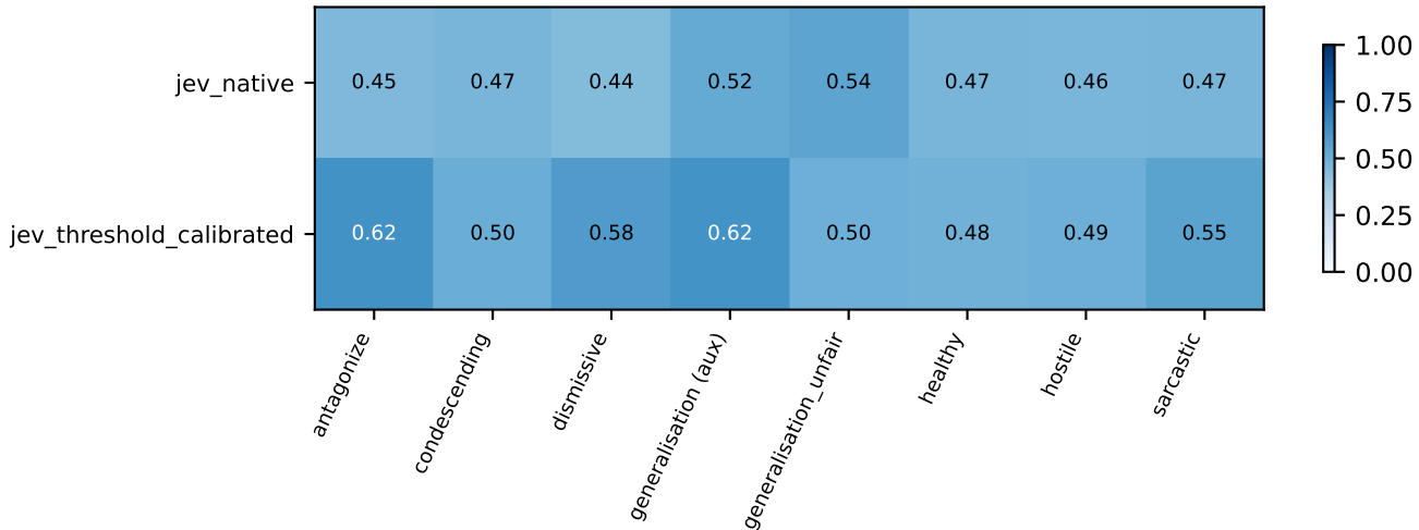
confirmation_jev_v1 / ucc / confirmation: Fixed-original-class macro F1
