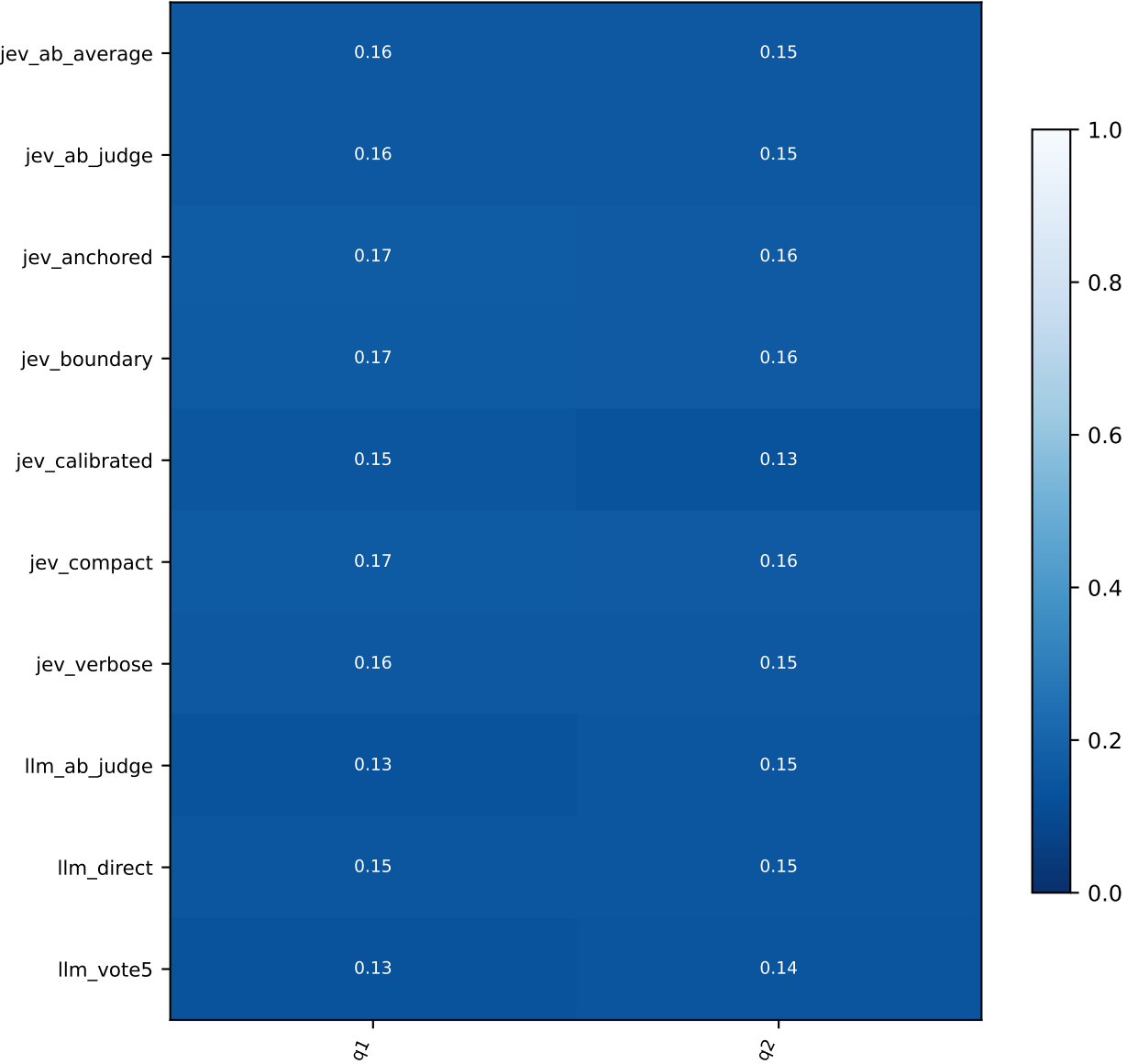
diagnostic_v1 / commonsense / diagnostic: Normalized MAE; original range retained in CSV
