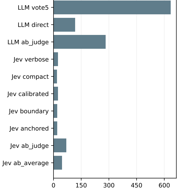
API latency sum, seconds (not wall)
