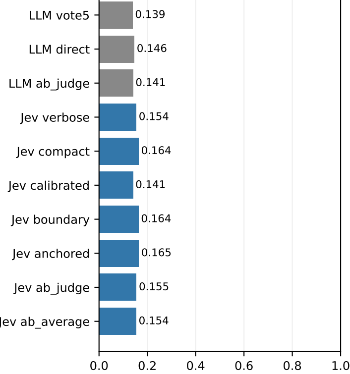
commonsense: Rater-fraction MAE (lower is better)
