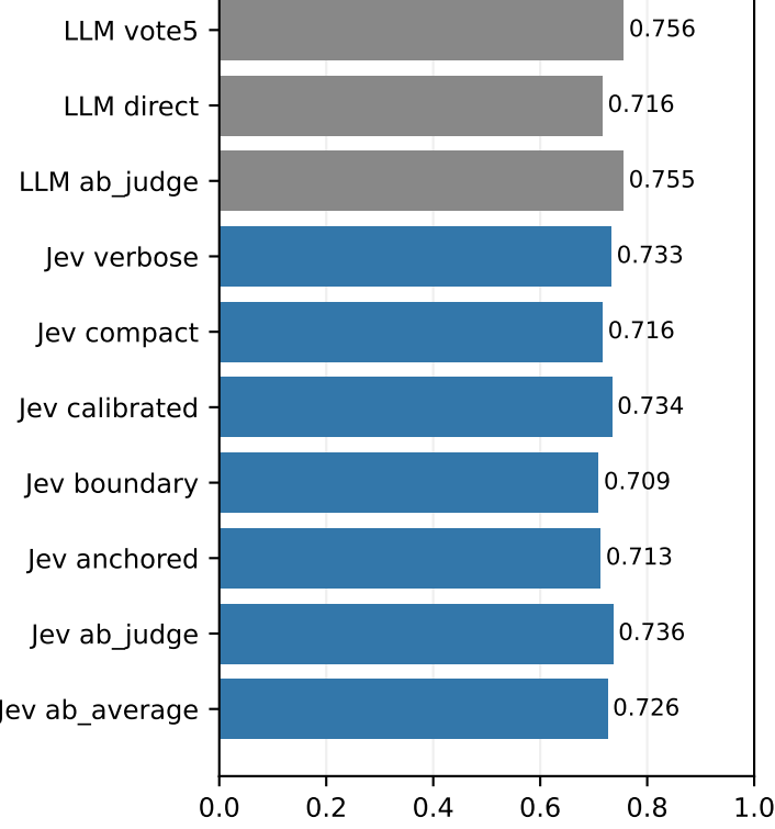
mbd: Original-class macro F1 (higher is better)
