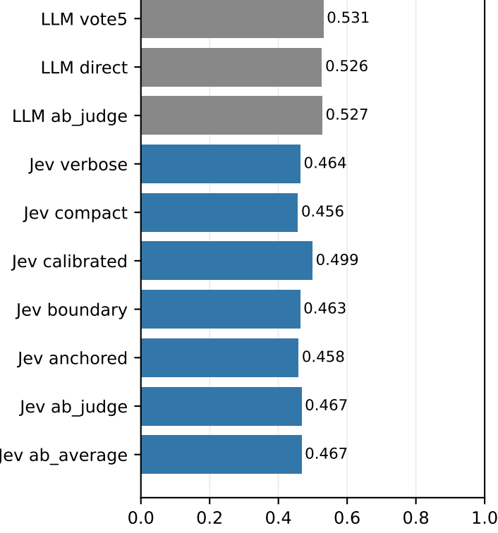
ucc: Original-class macro F1 (higher is better)
