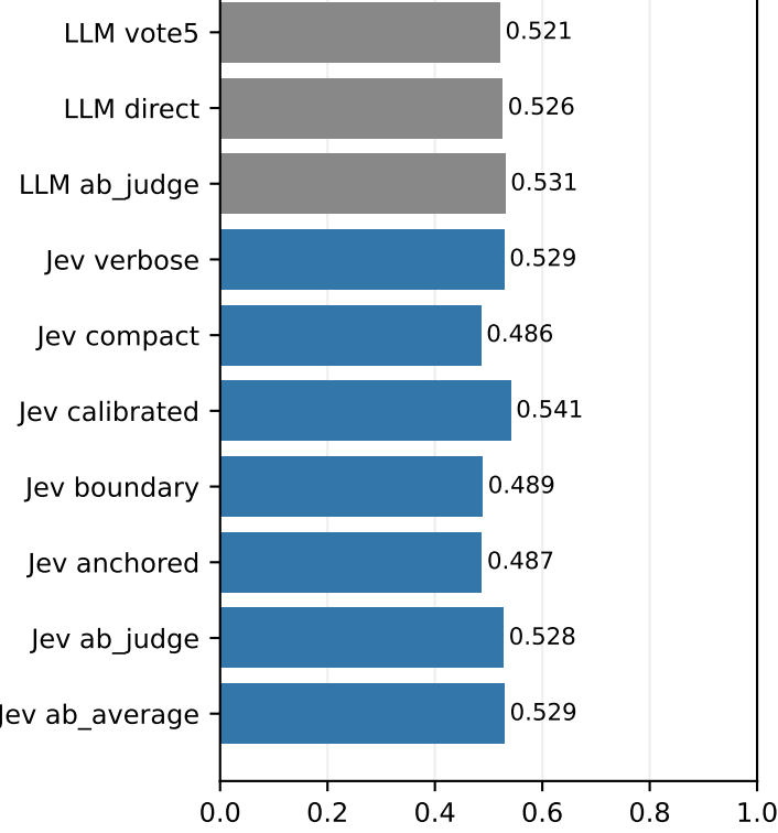
conflict: Original-class macro F1 (higher is better)
