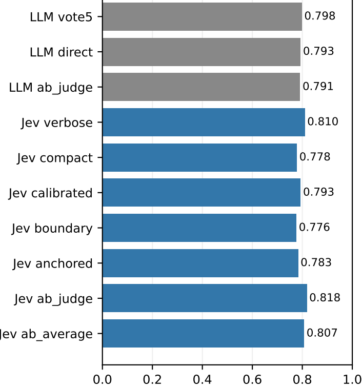
babe: Original-class macro F1 (higher is better)
