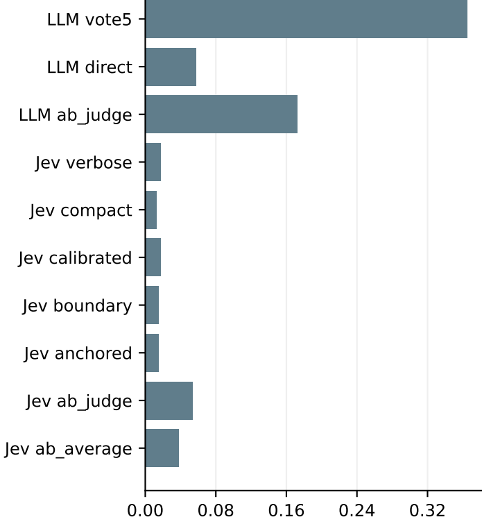
Standardized cold cost, USD (low rate)
