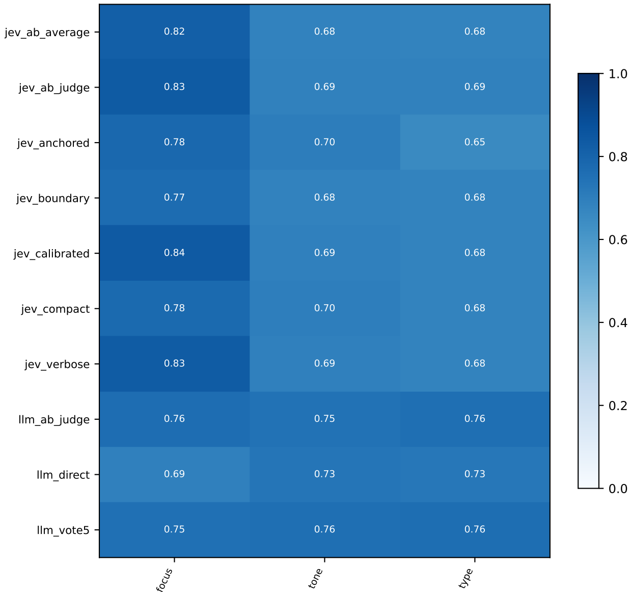
diagnostic_v1 / mbd / diagnostic: Fixed-original-class macro F1
