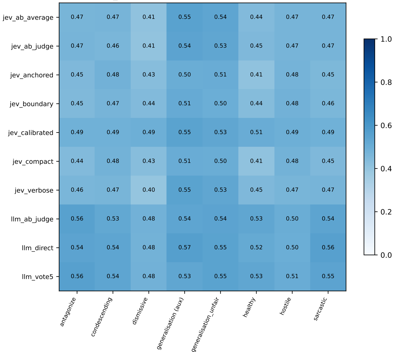
diagnostic_v1 / ucc / diagnostic: Fixed-original-class macro F1
