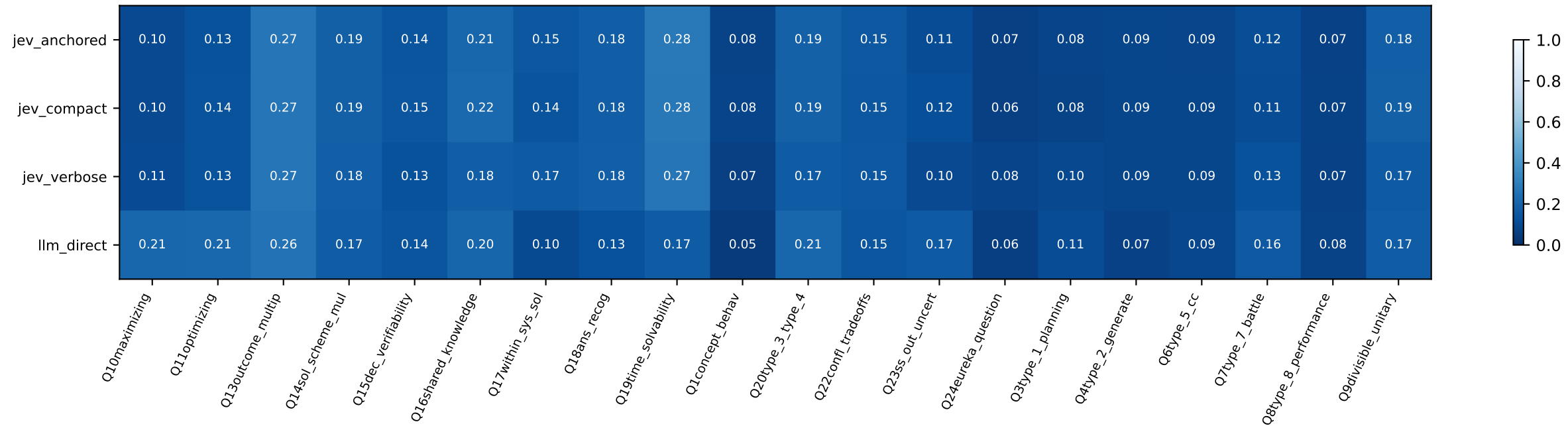
discovery_taskmap_v4 / taskmap / discovery: Normalized MAE; original range retained in CSV
