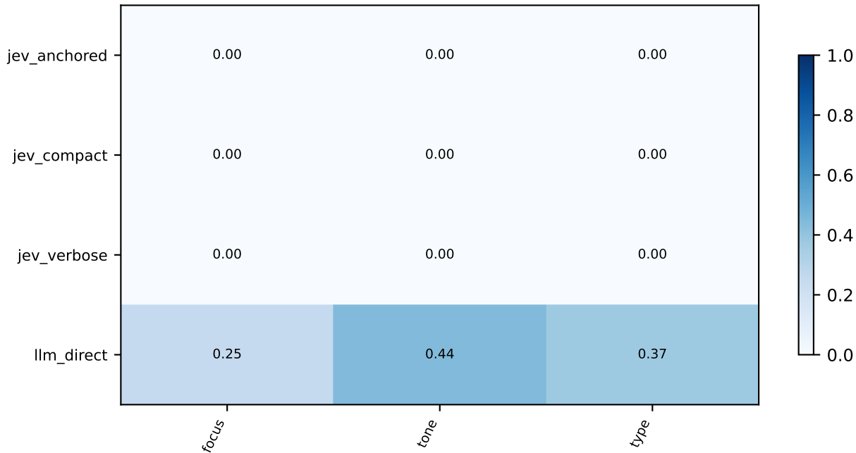
discovery_v1 / mbd / discovery: Fixed-original-class macro F1
