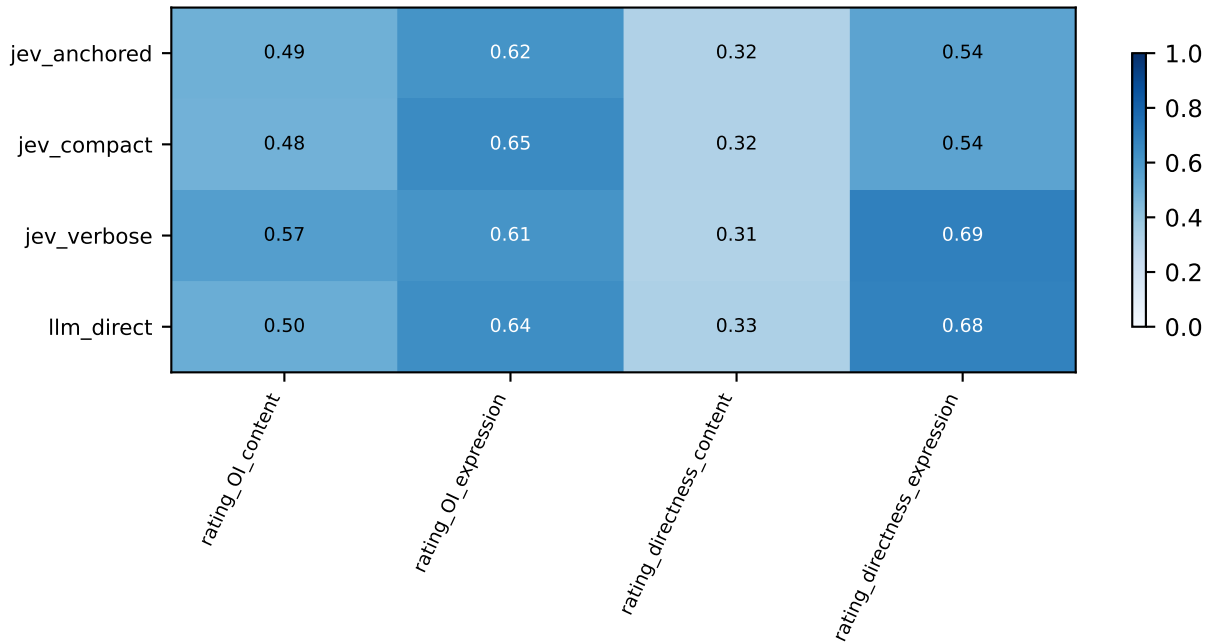
discovery_v2 / conflict / discovery: Fixed-original-class macro F1
