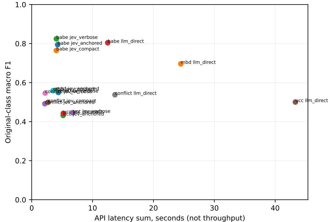
discovery_v2 efficiency-quality tradeoffs
