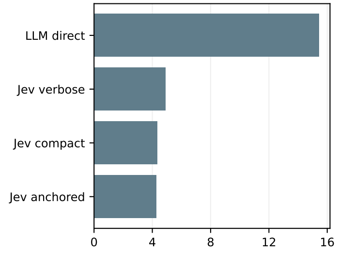
API latency sum, seconds (not wall)
