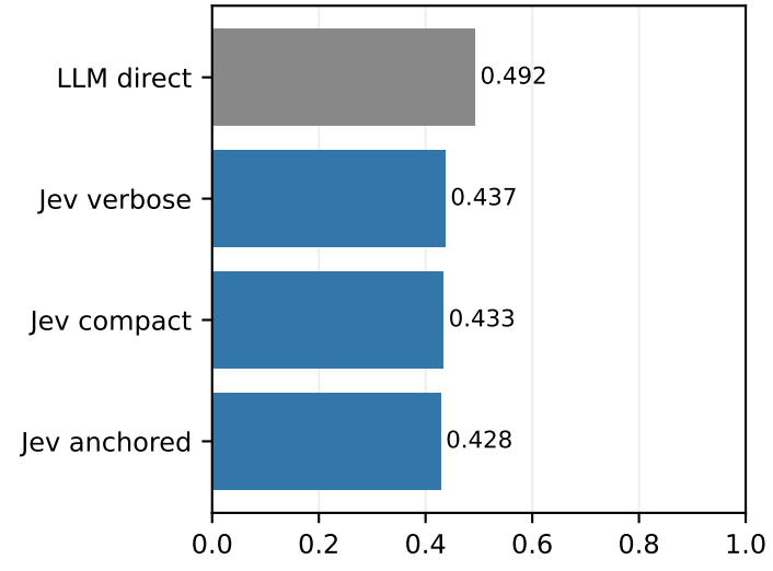
ucc: Original-class macro F1 (higher is better)
