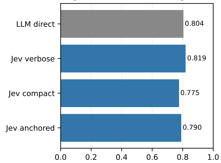
babe: Original-class macro F1 (higher is better)
