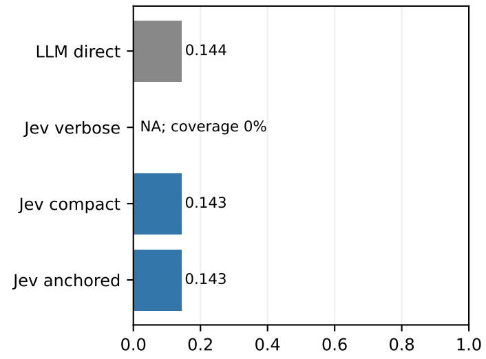
taskmap: Rater-fraction MAE (lower is better)
