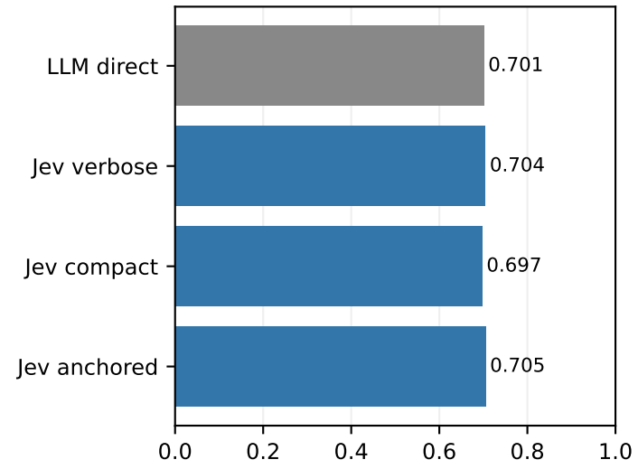
mbd: Original-class macro F1 (higher is better)
