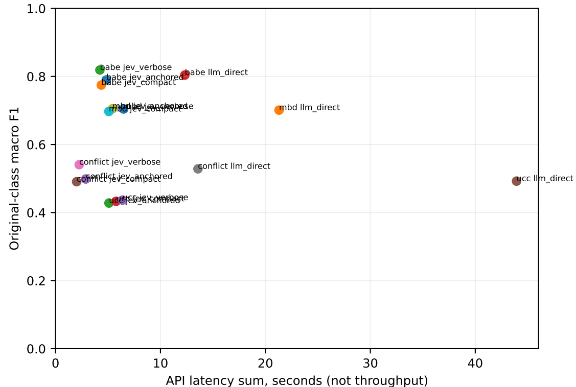
discovery_v3 efficiency-quality tradeoffs
