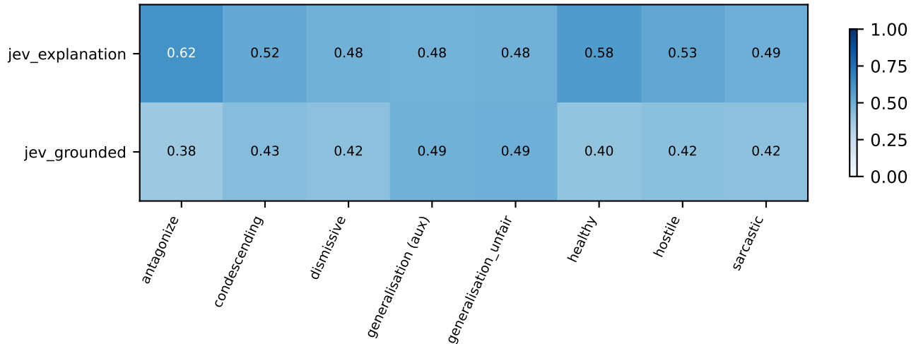
explanation_discovery_v2 / ucc / discovery: Fixed-original-class macro F1
