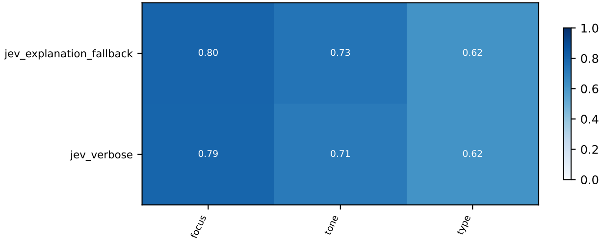
explanation_fallback_discovery_v3 / mbd / discovery: Fixed-original-class macro F1
