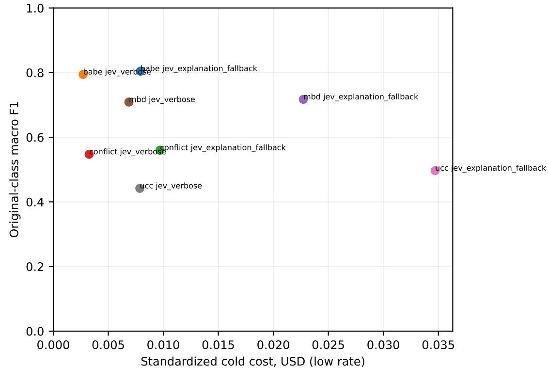
explanation_fallback_discovery_v3 efficiency-quality tradeoffs
