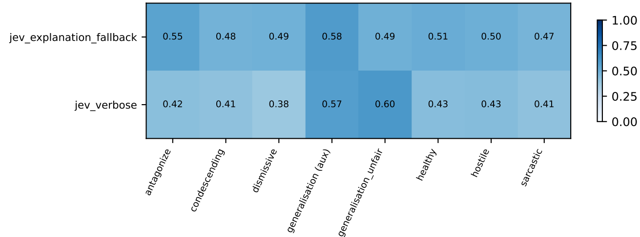
explanation_fallback_discovery_v3 / ucc / discovery: Fixed-original-class macro F1
