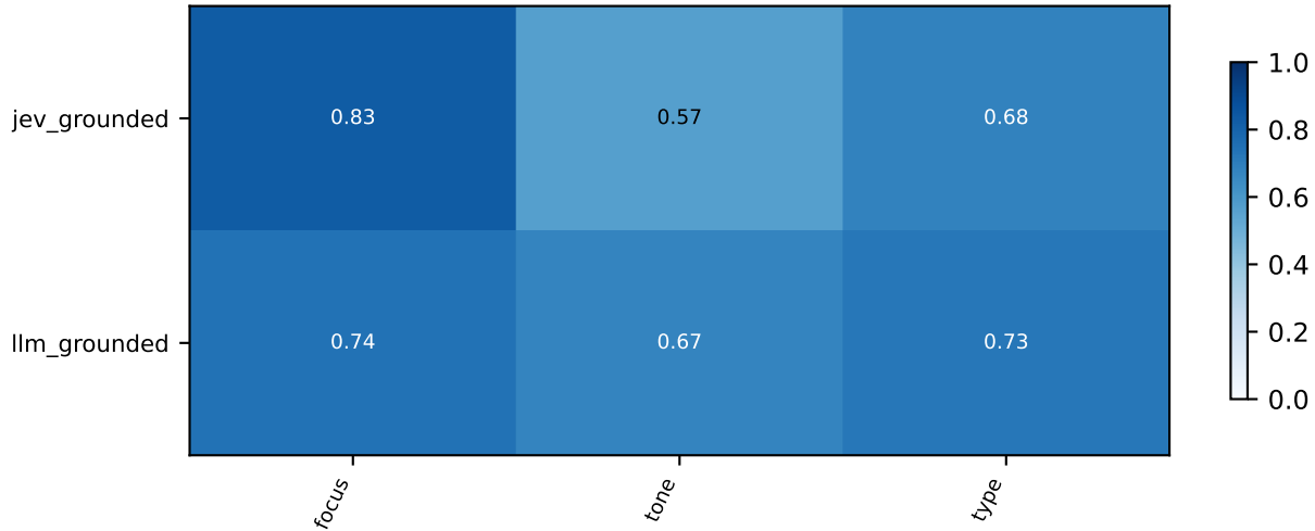
grounded_calibration_v1 / mbd / calibration: Fixed-original-class macro F1
