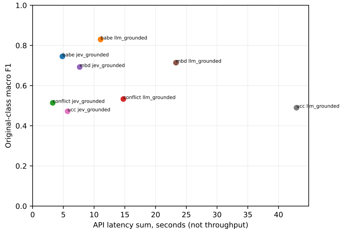
grounded_calibration_v1 efficiency-quality tradeoffs
