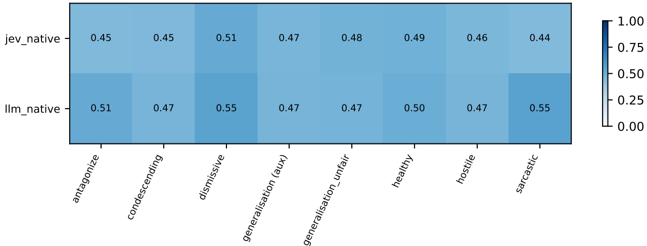
native_calibration_v1 / ucc / calibration: Fixed-original-class macro F1
