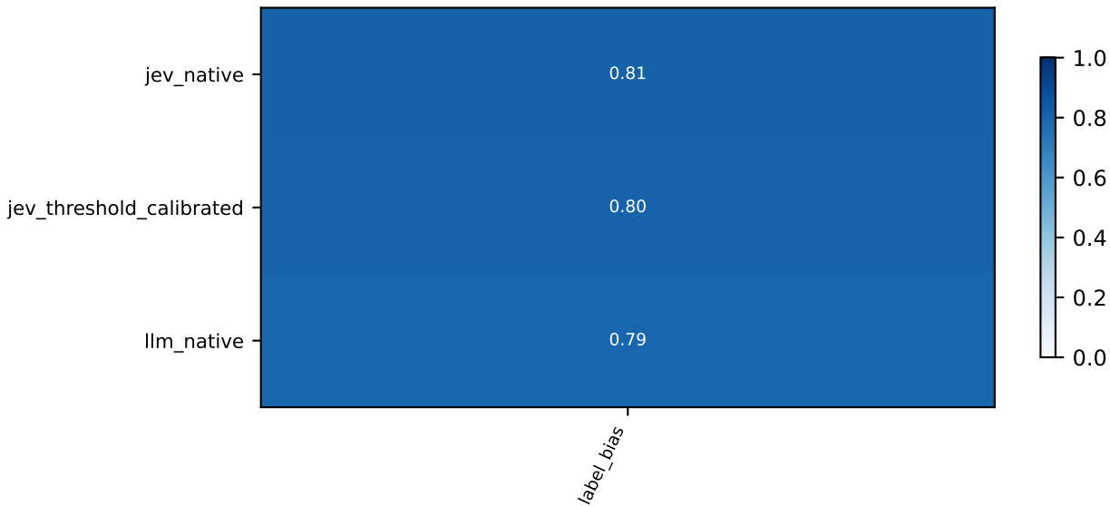
native_diagnostic_v1 / babe / diagnostic: Fixed-original-class macro F1
