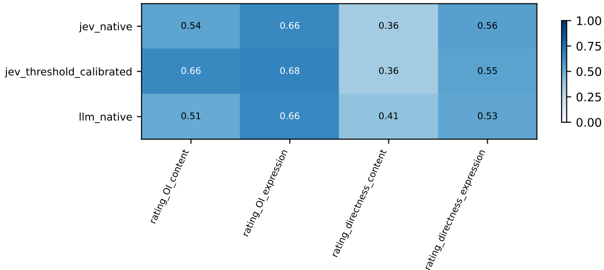
native_diagnostic_v1 / conflict / diagnostic: Fixed-original-class macro F1
