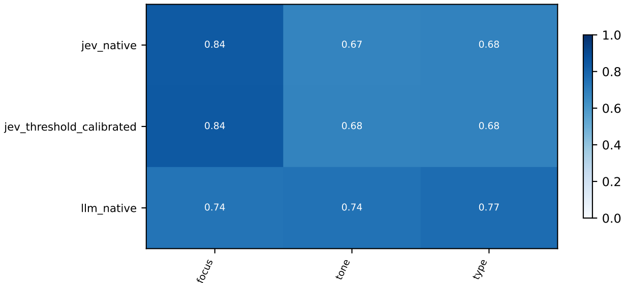
native_diagnostic_v1 / mbd / diagnostic: Fixed-original-class macro F1
