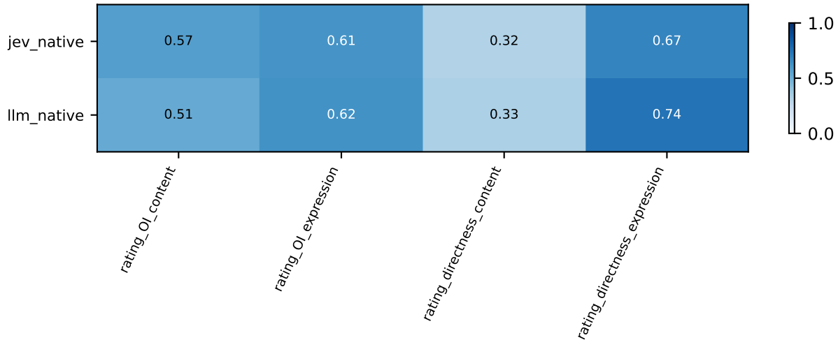
native_discovery_v1 / conflict / discovery: Fixed-original-class macro F1
