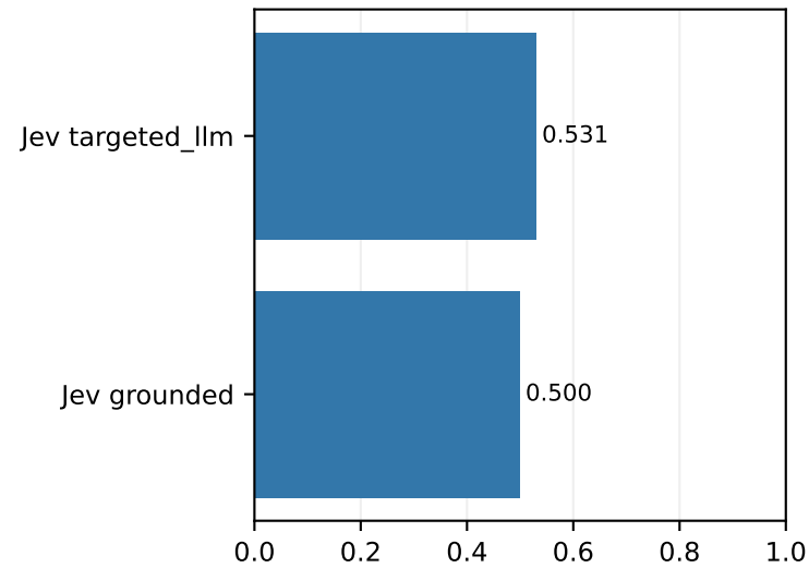
conflict: Original-class macro F1 (higher is better)
