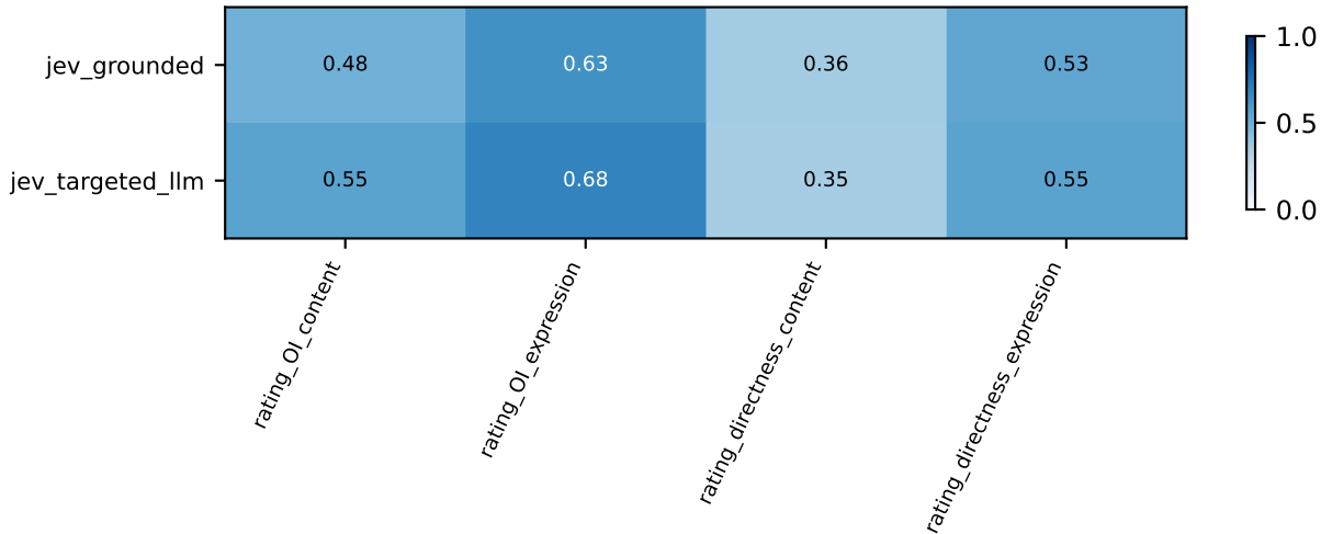
routing_diagnostic_v1_b025 / conflict / diagnostic: Fixed-original-class macro F1
