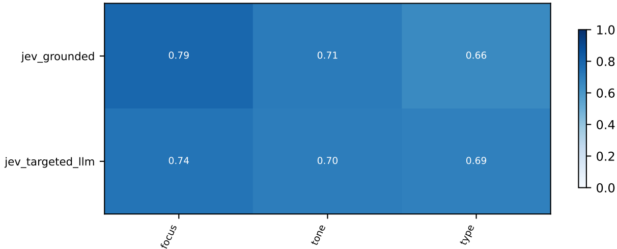
routing_diagnostic_v1_b025 / mbd / diagnostic: Fixed-original-class macro F1
