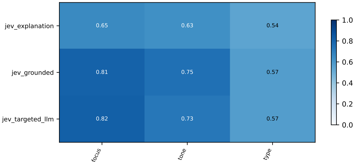
routing_discovery_v1_b025 / mbd / discovery: Fixed-original-class macro F1
