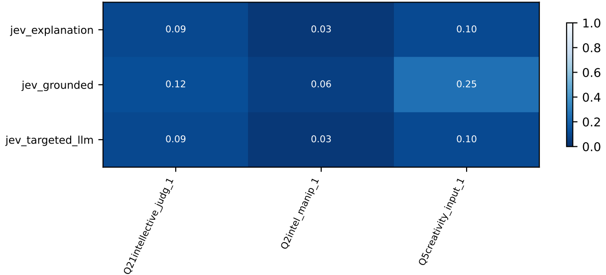
routing_discovery_v1_b025 / taskmap / discovery: Normalized MAE; original range retained in CSV
