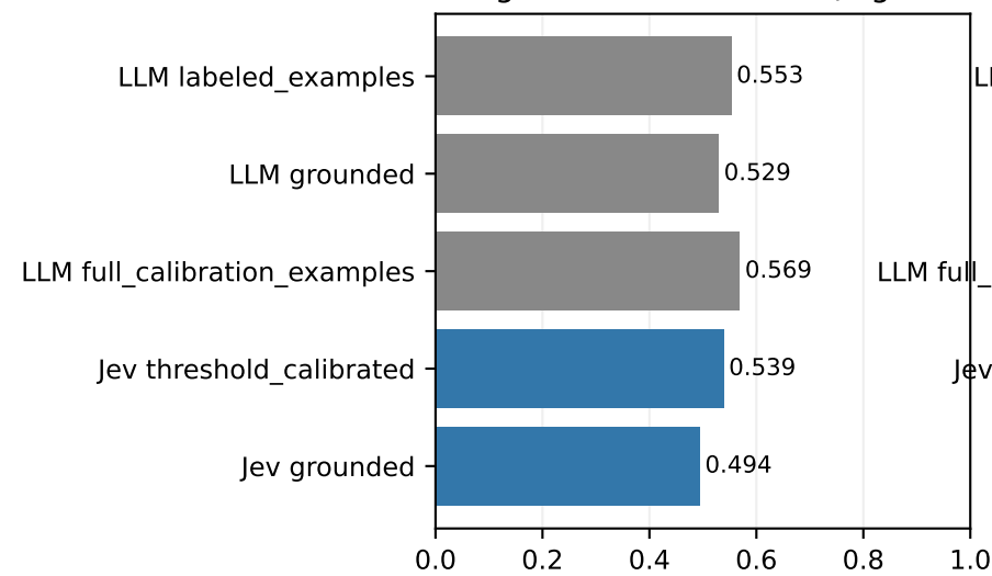
conflict: Original-class macro F1 (higher is better)
