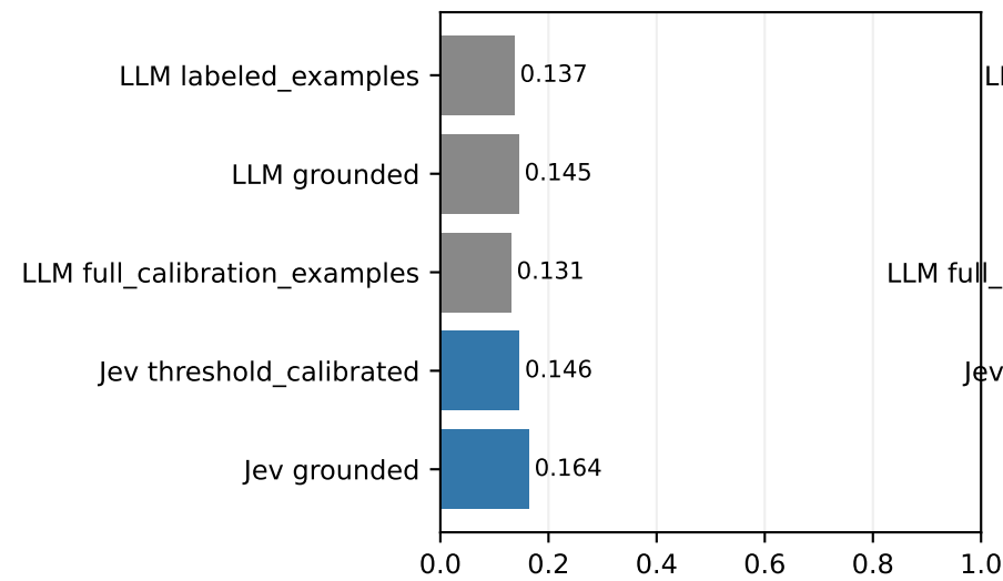
commonsense: Rater-fraction MAE (lower is better)
