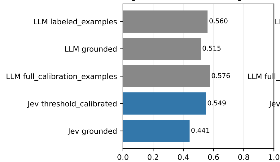
ucc: Original-class macro F1 (higher is better)
