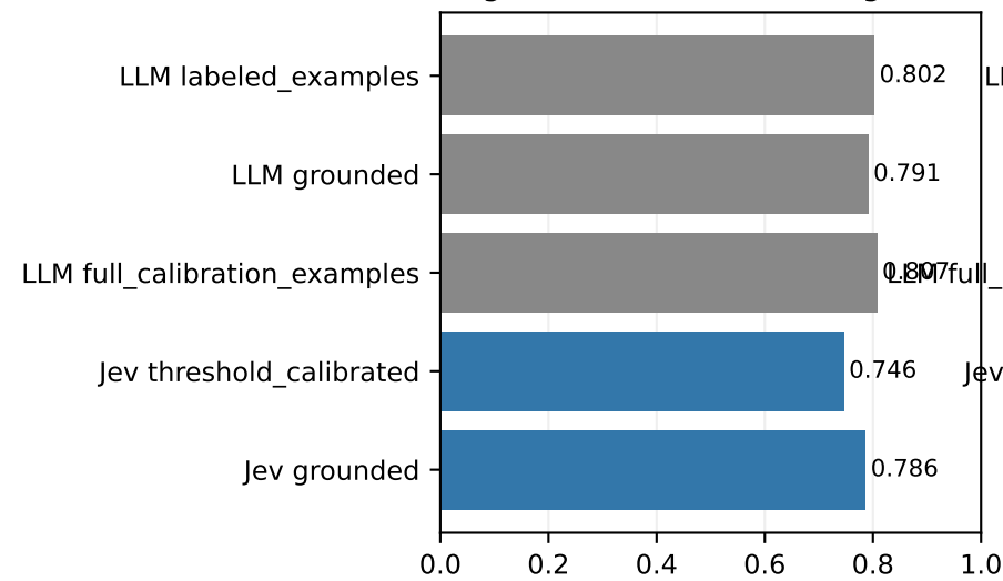
babe: Original-class macro F1 (higher is better)
