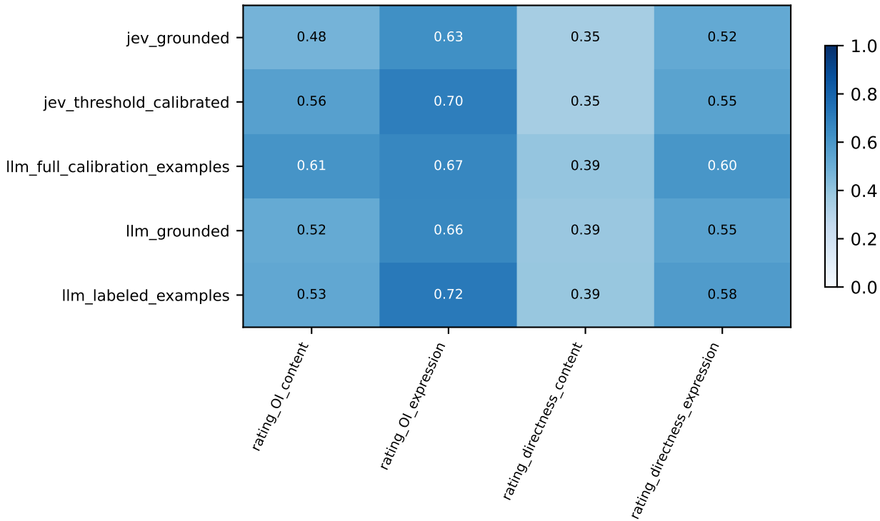
strengthening_diagnostic_v1 / conflict / diagnostic: Fixed-original-class macro F1
