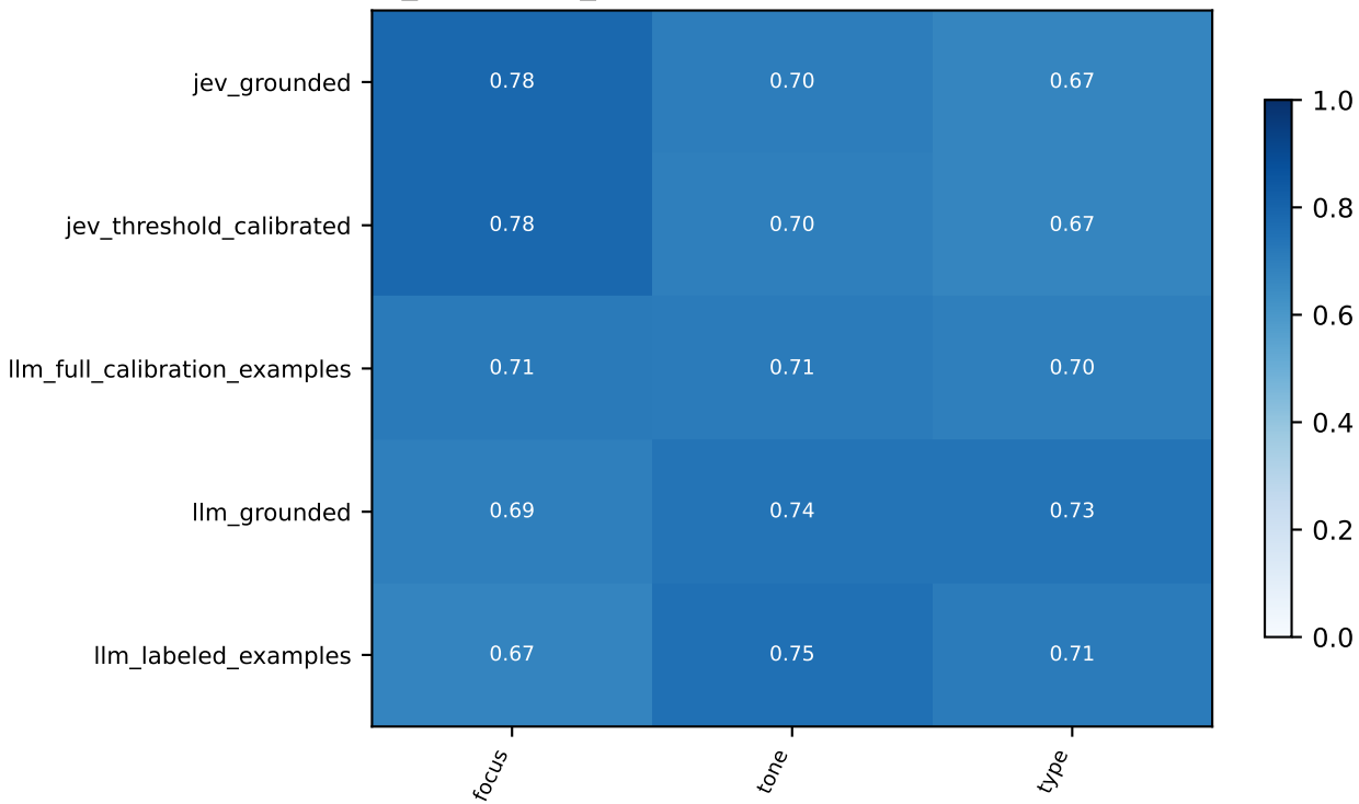
strengthening_diagnostic_v1 / mbd / diagnostic: Fixed-original-class macro F1
