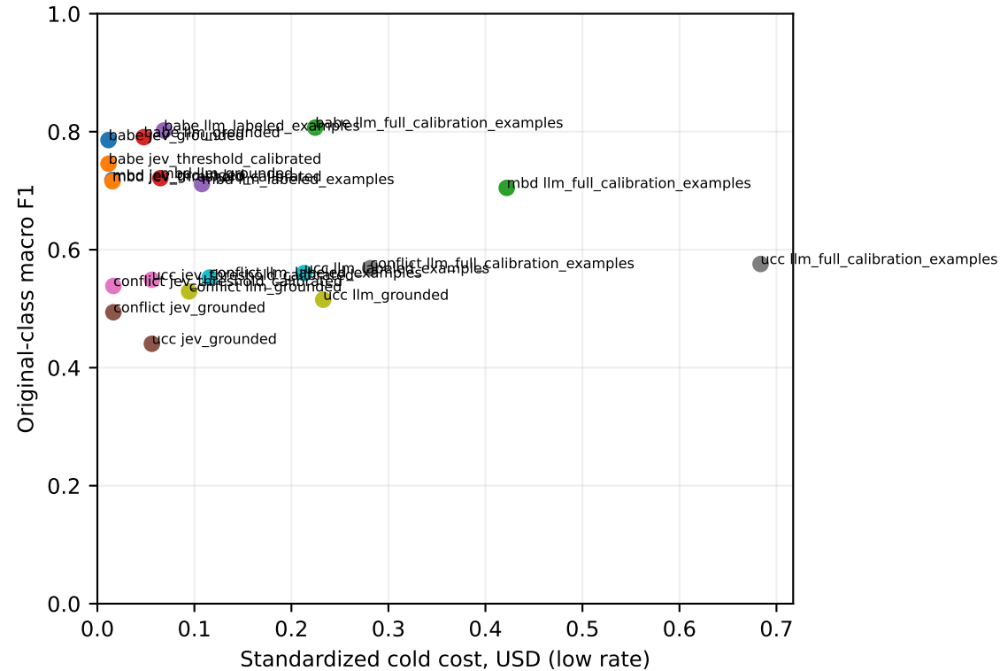
strengthening_diagnostic_v1 efficiency-quality tradeoffs
