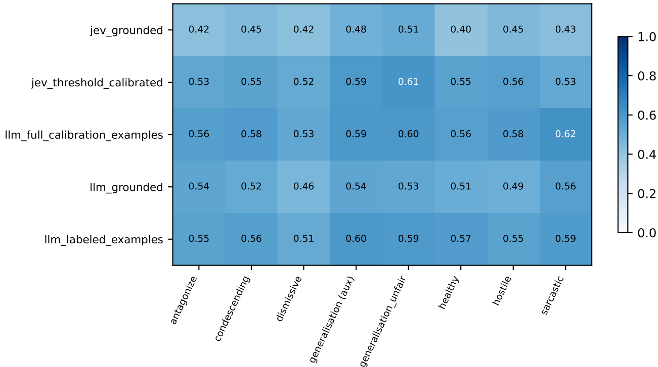
strengthening_diagnostic_v1 / ucc / diagnostic: Fixed-original-class macro F1
