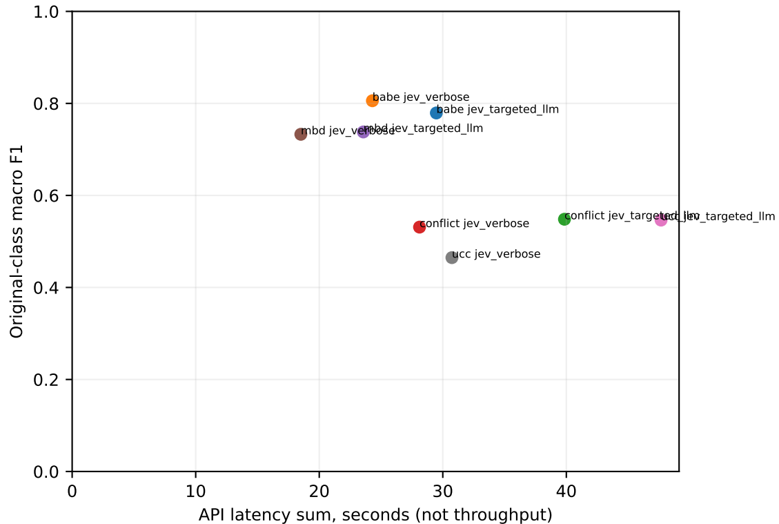
verbose_routing_diagnostic_v1_b01 efficiency-quality tradeoffs
