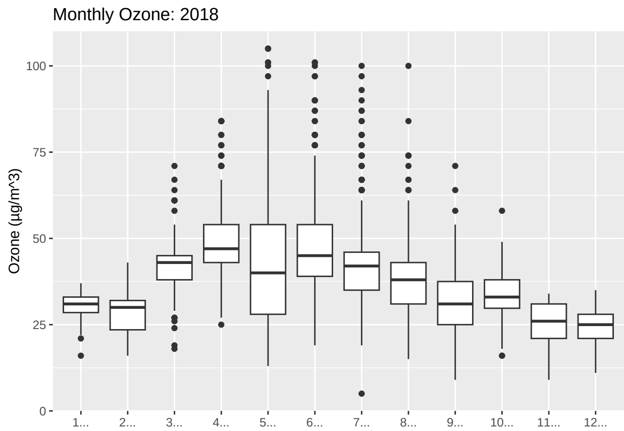
Figure 1: Monthly Ozone (2018)
