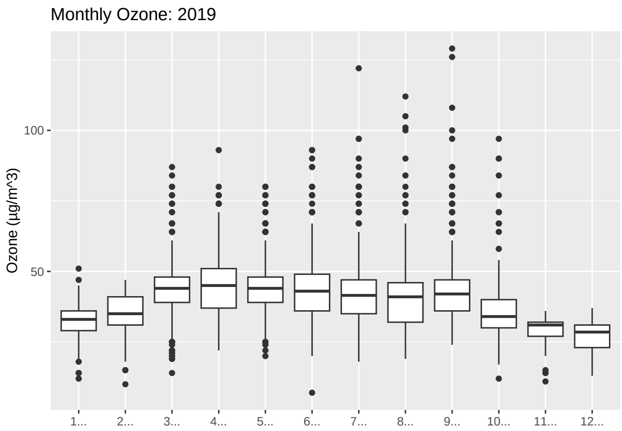
Figure 2: Monthly Ozone (2019)
