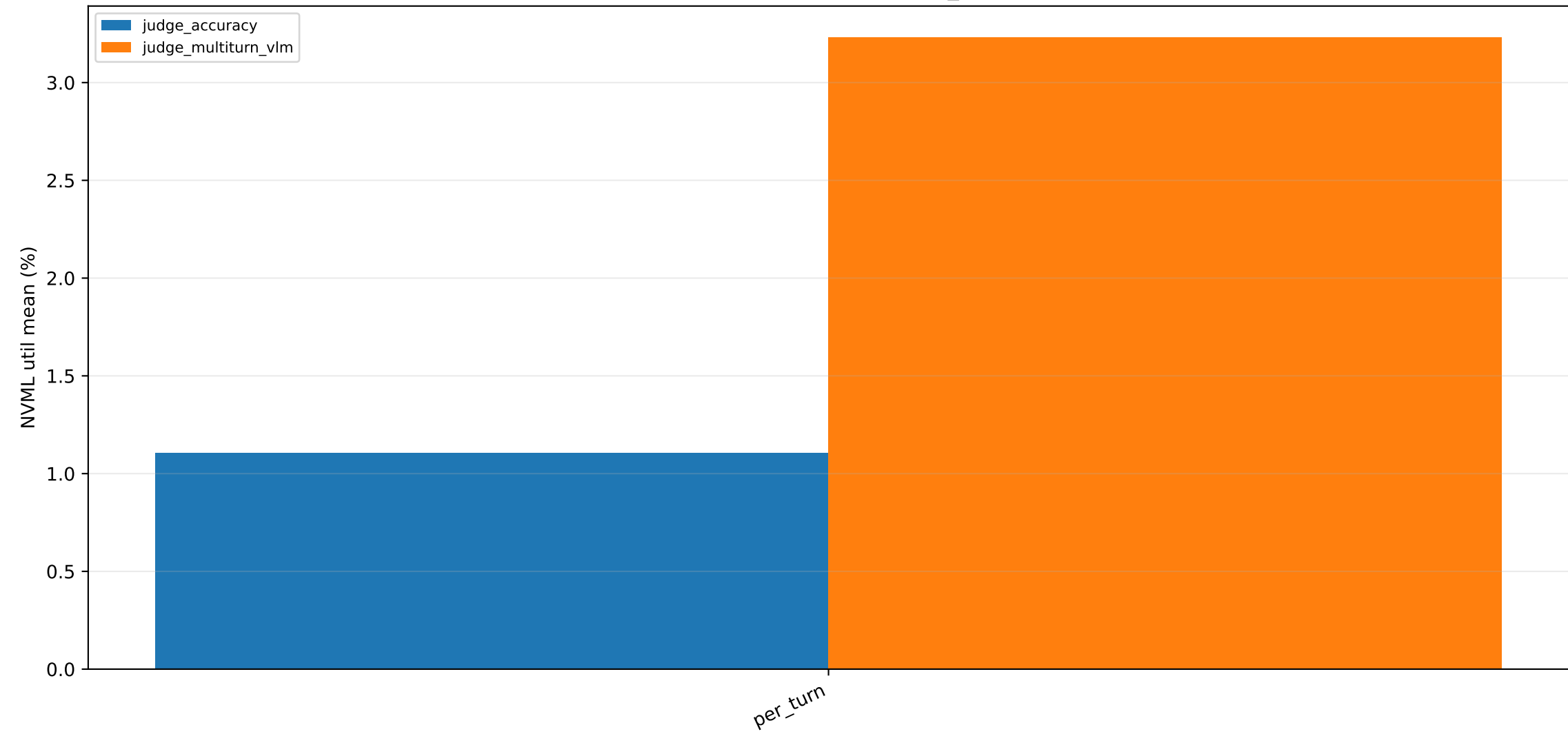
Reward GPU utilization (per_turn)
