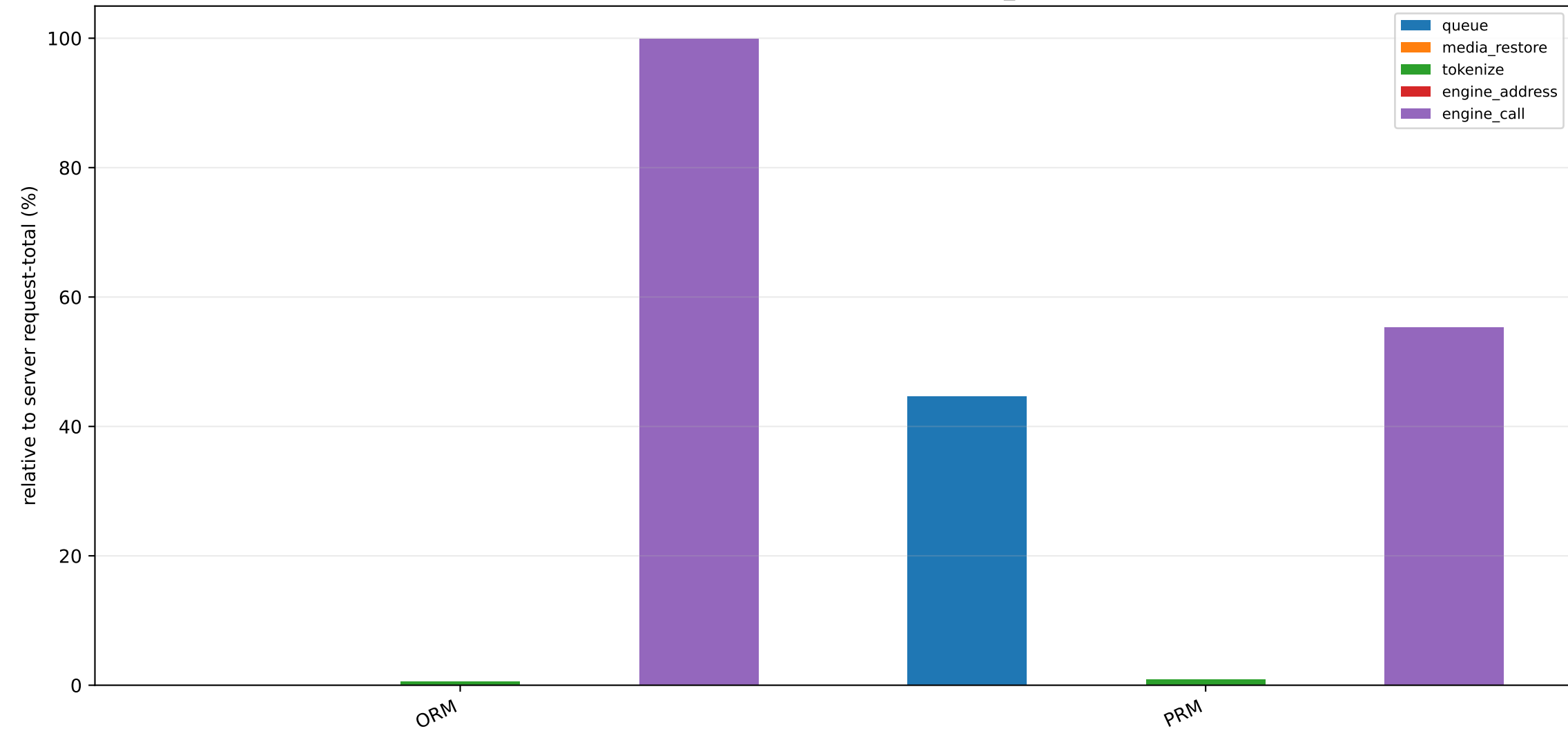
Reward server-side components (per_turn)
