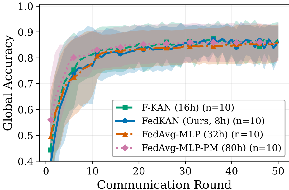
Multiclass — Dirichlet \alpha = 0.1
