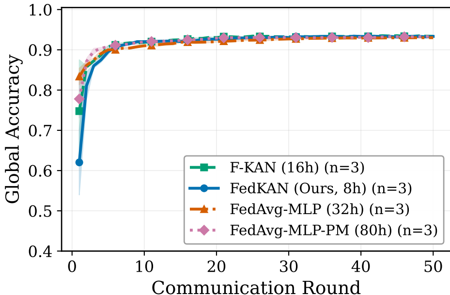
Multiclass — Dirichlet \alpha = 1.0
