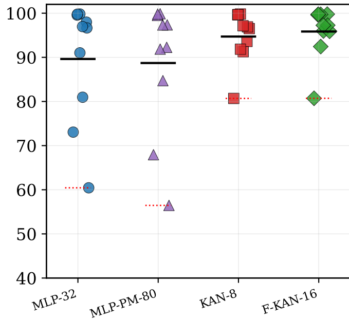
(a) NF-BoT-IoT-v2 (high skew)
