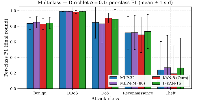
Fig. 4. Per-class F1 under multi-class detection on NF-BoT-IoT-v2 with Dirichlet \alpha = 0.1 ( n = 10 seeds). Bars show mean F1; error bars are \pm 1 std. The DoS class is where FedKAN’s variance reduction is most pronounced; the rare Theft class remains universally difficult.
