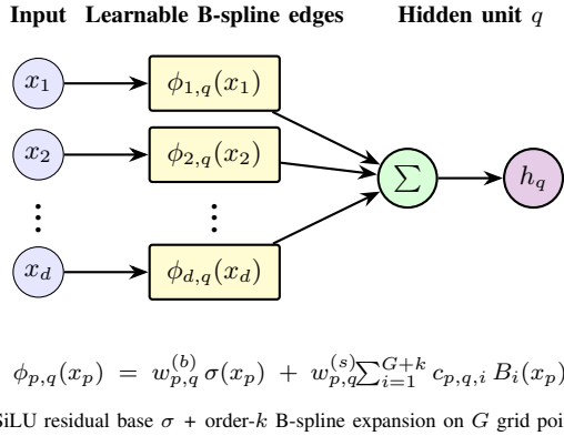
Fig. 2. Sub-flow: structure of one KAN layer producing hidden unit h_q from input vector \mathbf{x} \in \mathbb{R}^d . Each edge (p, q) carries an independent learnable activation \phi_{p,q} parameterised as a SiLU residual base plus a B-spline expansion on a uniform grid of G points (order k ). The full client model stacks an input layer ( d \rightarrow n_h ) and an output layer ( n_h \rightarrow c ). The B-spline coefficients c_{p,q,i} have local support.
