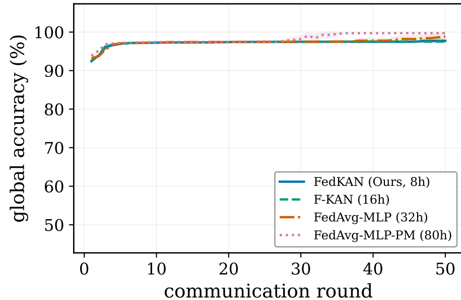
(a) IID n = 10
