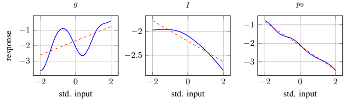
Fig. 4. Extracted univariate rules (solid) and best-fit closed form (dashed). The p_0 and I dependences are near-linear; g is nonlinear and carried by the spline.
