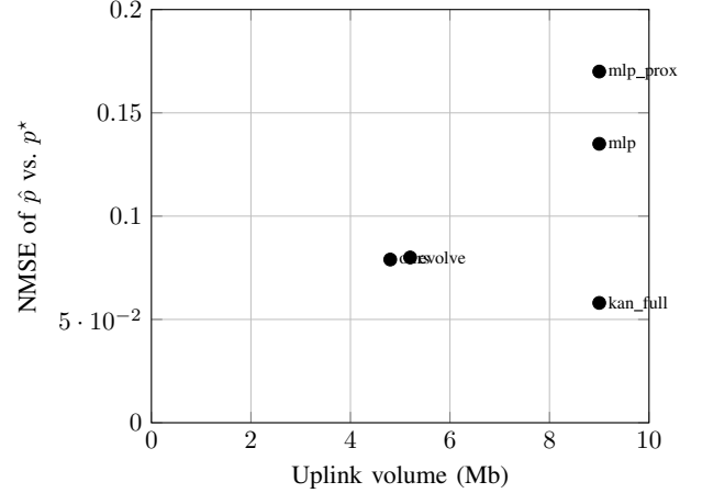
Fig. 1. Communication-accuracy frontier. The proposed bandit-sparsified KAN (ours) dominates both MLP variants and halves the uplink of the dense KAN.
