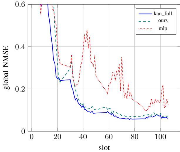
Fig. 3. Global NMSE over the non-stationary horizon (representative seed).
