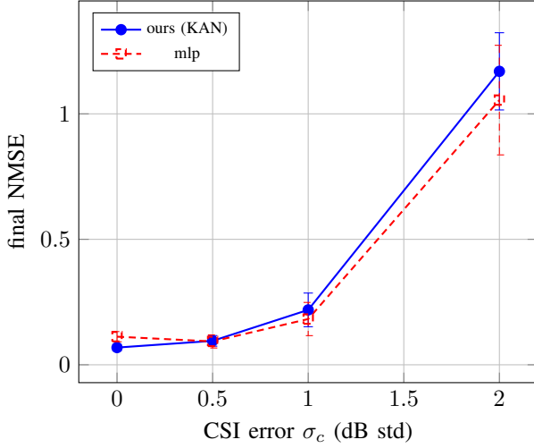
Fig. 10. Robustness to CSI estimation error in the federated loop. The KAN leads at small error; the methods converge as the error grows and the input becomes uninformative.
